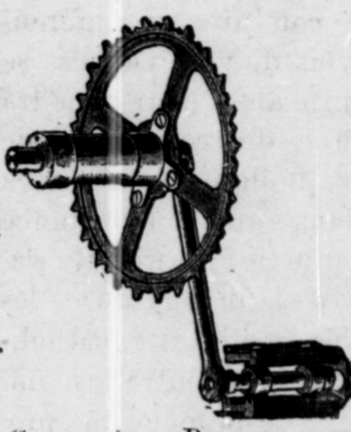
CRANK AXLE BEARING WITH IMPROVED CASE REMOVED FROM BRACKET
