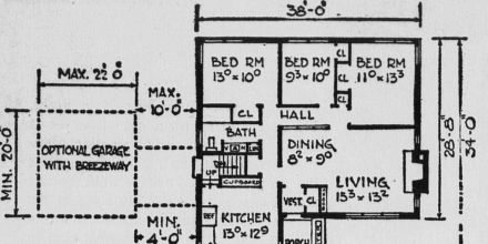
Design No. 609 1196 Sq. Ft. Blueprints include complete details for building in either Brick or Frame.
