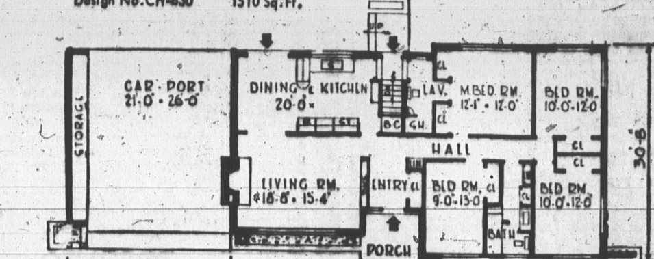
Design No. CH-630 1510 Sq. Ft.
