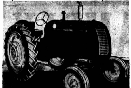
COCKSHUTT 30 DELUXE 33 Belt H.P.; 28.5 Draw Bar H.P.; Live Power Take-off; 8 forward speeds; 4 Way live hydraulic system; 4 types of interchangeable front ends; 3 pt. hitch; gas or diesel.
