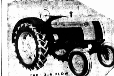
COCKSHUTT 40 DELUXE 47 Belt H.P.; 42 Draw Bar H.P.; Live Power Take-Off; 7 Bearing Crankshaft; double wall final drive; 3 pt. hitch; D4 or D6 Diesel or gas.
