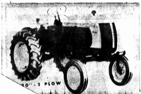
COCKSHUTT 20 DELUXE 30.4 Belt H.P.; 26.75 Draw Bar H.P.; 2 Types of Front Ends; 4-way live hydraulic system; 11" tires for better traction; 3 pt. hitch.
