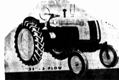
COCKSHUTT 35 DELUXE 36 1/2 Draw Bar H.P.; 42 Belt H.P.; Live Power Take-Off; 4 Way live hydraulic system; 5 bearing crankshaft; power steering; 3 pt. hitch; Gas or diesel.
