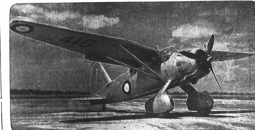
The Westland Lysander, shown above, which is being built by the National Steel Car Co., at its new aircraft plant at Malton, for the R.C.A.F., is a single-engine two-seat army co-operation high wing monoplane. It is one of the most popular planes in the Royal Air Force. The cockpit is in front of and level with the leading edge of the wings, so as to provide the pilot with exceptional view, while there is provision for machine guns and bomb racks. It is powered with a Bristol Mercury, XII nine-cylinder radial air-cooled engine and has a maximum speed of 220 miles per hour. It is credited with a quick take off, low landing speed and a steep climb. The Malton plant is also being used for the construction of British aircraft under the Canadian Associated Aircrafts scheme. The building has now been completed. Delivery of these Lysander planes, for the Royal Canadian Air Force are now being made.
