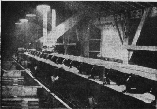
Shuttle Conveyor for filling storage bins and for bulk delivery
