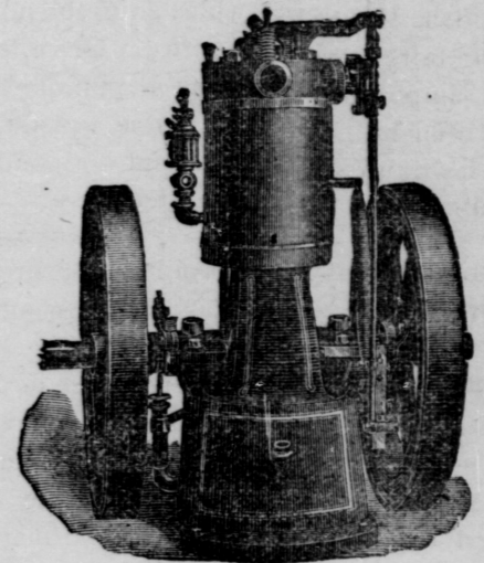
Vertical Gas or Gasoline Engine, 1, 2 & 4 Horse-Power
